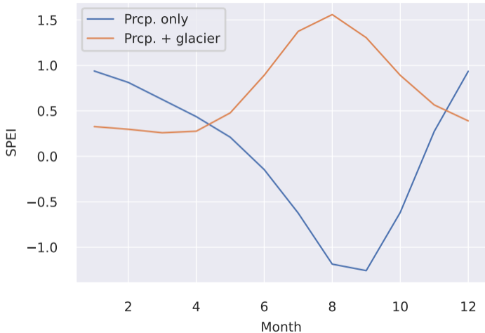
Mean annual cycle of SPEI in the Copper basin, N. America
