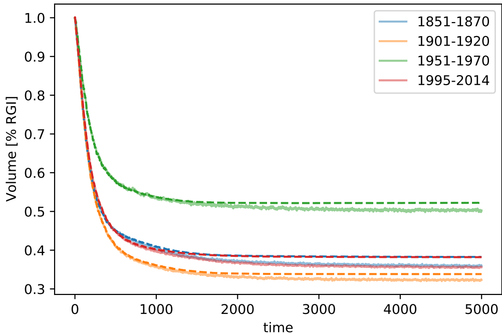
RGI07 (dash=stop). Stop crit 2 (SMB based, 100 yr period)
