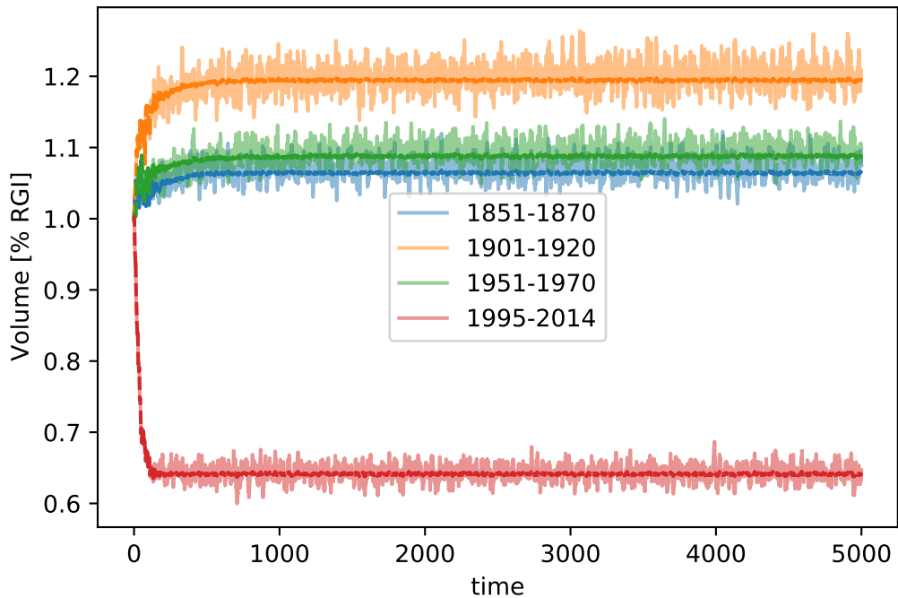
RGI15 (dash=stop). Stop crit 2 (SMB based, 100 yr period)
