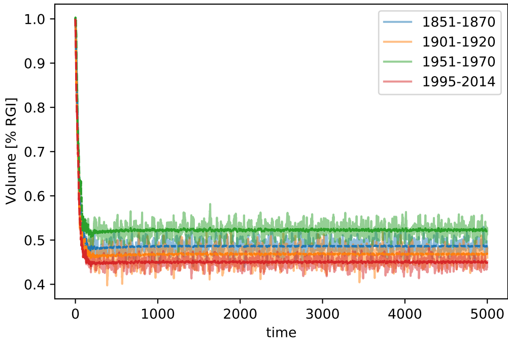
RGI11 (dash=stop). Stop crit 2 (SMB based, 100 yr period)
