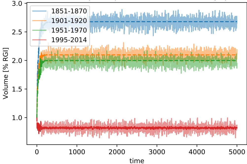
RGI16 (dash=stop). Stop crit 2 (SMB based, 100 yr period)
