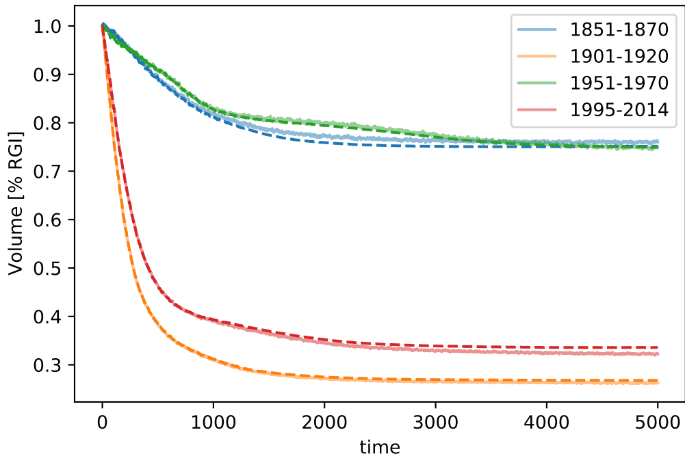
RGI19 (dash=stop). Stop crit 2 (SMB based, 100 yr period)
