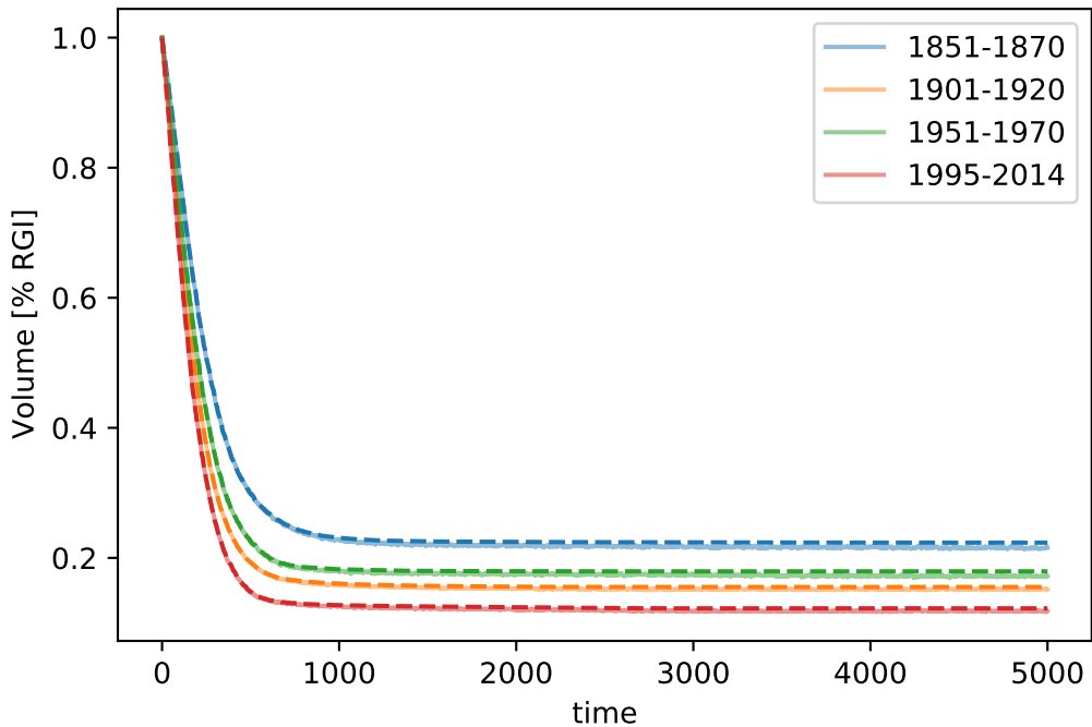
RGI04 (dash=stop). Stop crit 2 (SMB based, 100 yr period)
