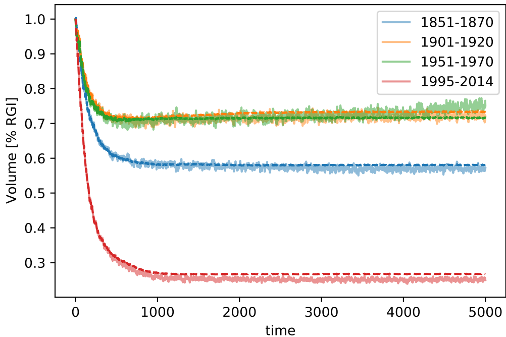
RGI08 (dash=stop). Stop crit 2 (SMB based, 100 yr period)
