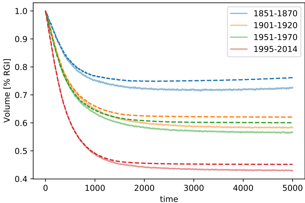
RGI03 (dash=stop). Stop crit 2 (SMB based, 100 yr period)
