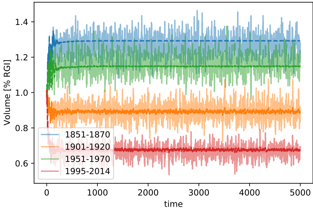
RGI18 (dash=stop). Stop crit 2 (SMB based, 100 yr period)
