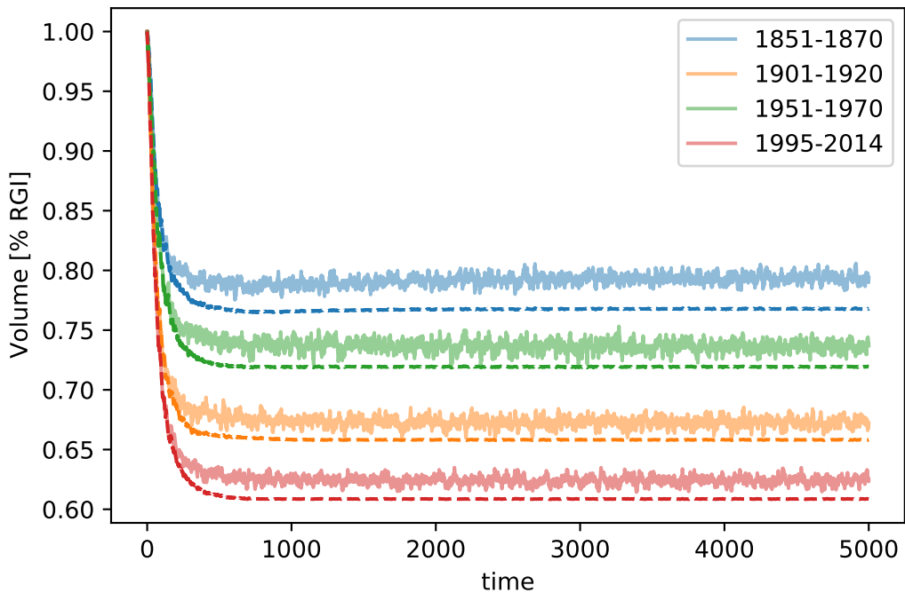
RGI01 (dash=stop). Stop crit 2 (SMB based, 100 yr period)
