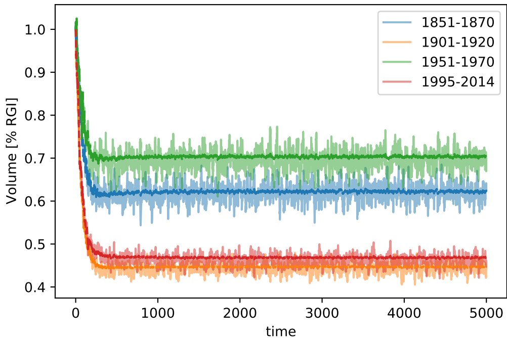
RGI02 (dash=stop). Stop crit 2 (SMB based, 100 yr period)
