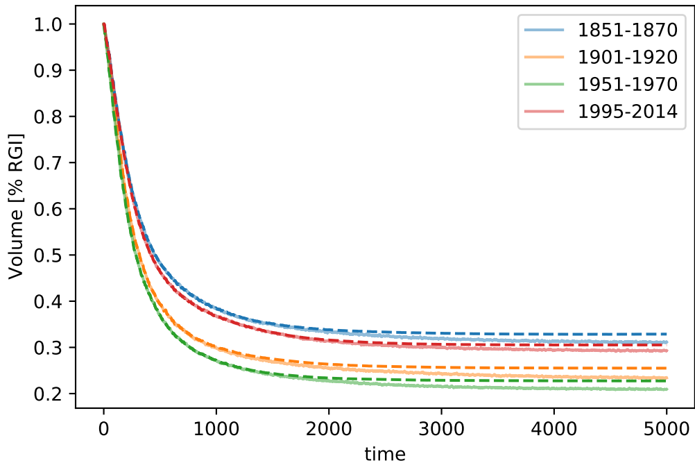
RGI09 (dash=stop). Stop crit 2 (SMB based, 100 yr period)
