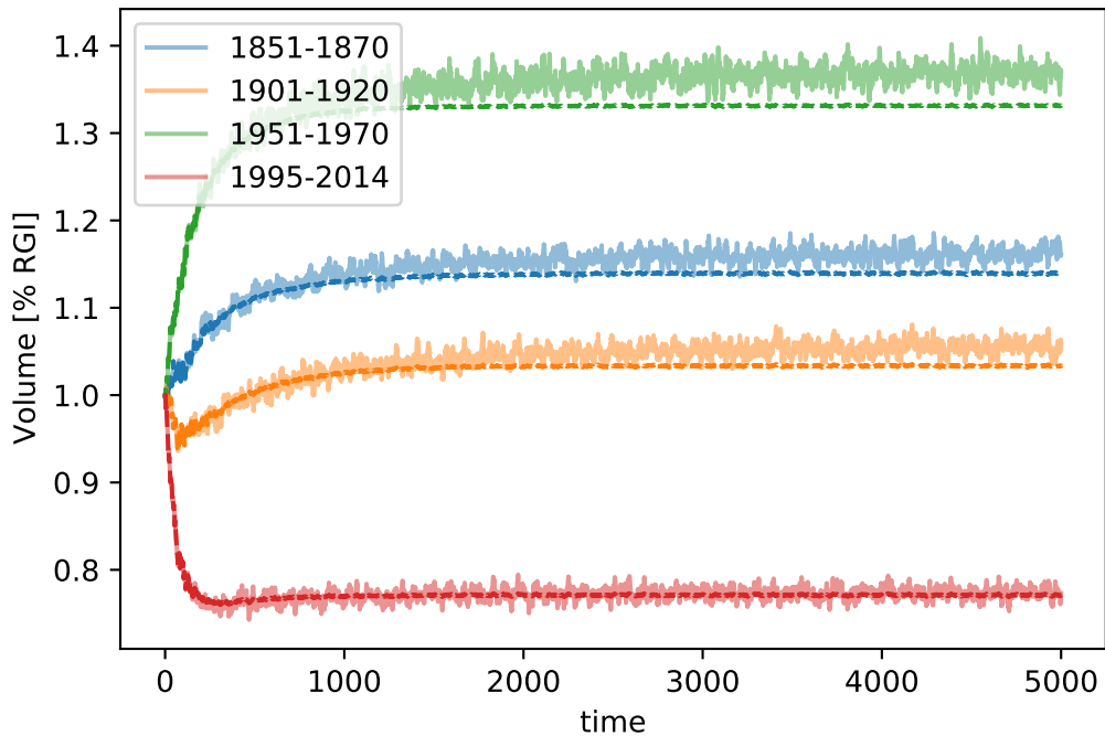
RGI13 (dash=stop). Stop crit 2 (SMB based, 100 yr period)
