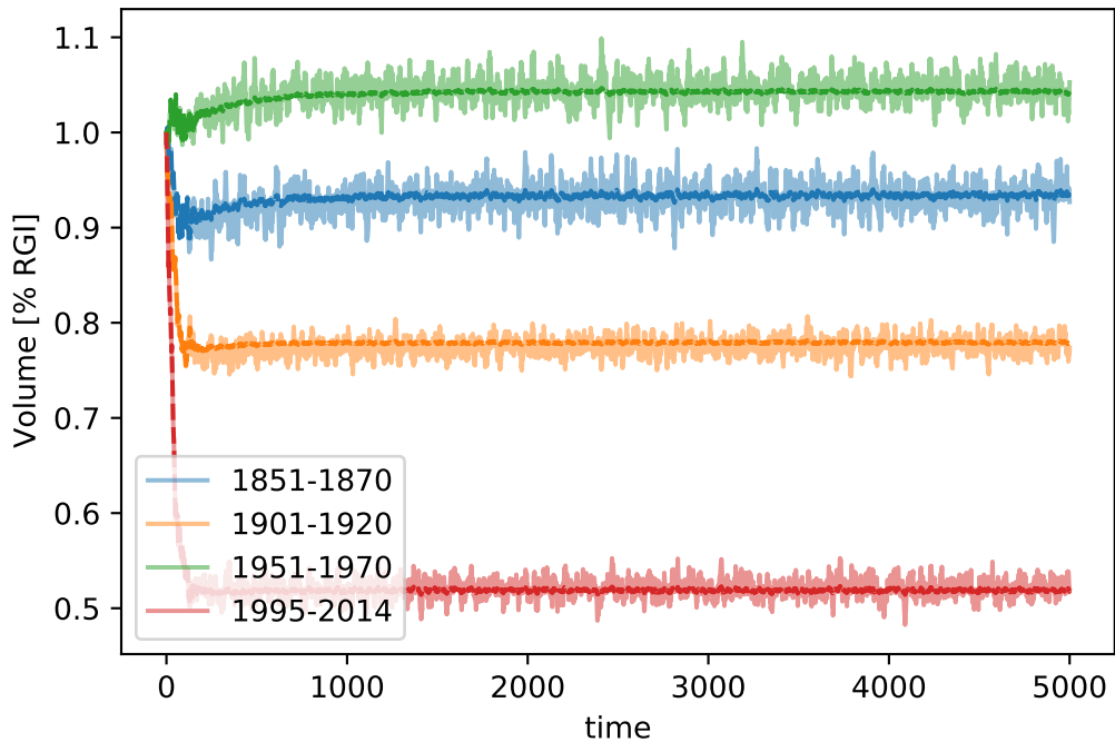
RGI12 (dash=stop). Stop crit 2 (SMB based, 100 yr period)
