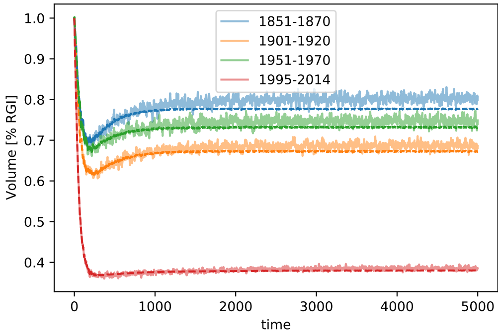
RGI10 (dash=stop). Stop crit 2 (SMB based, 100 yr period)
