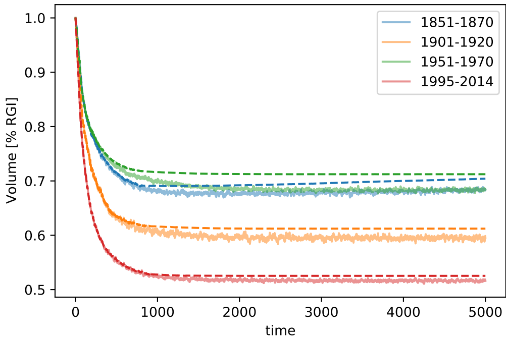
RGI06 (dash=stop). Stop crit 2 (SMB based, 100 yr period)
