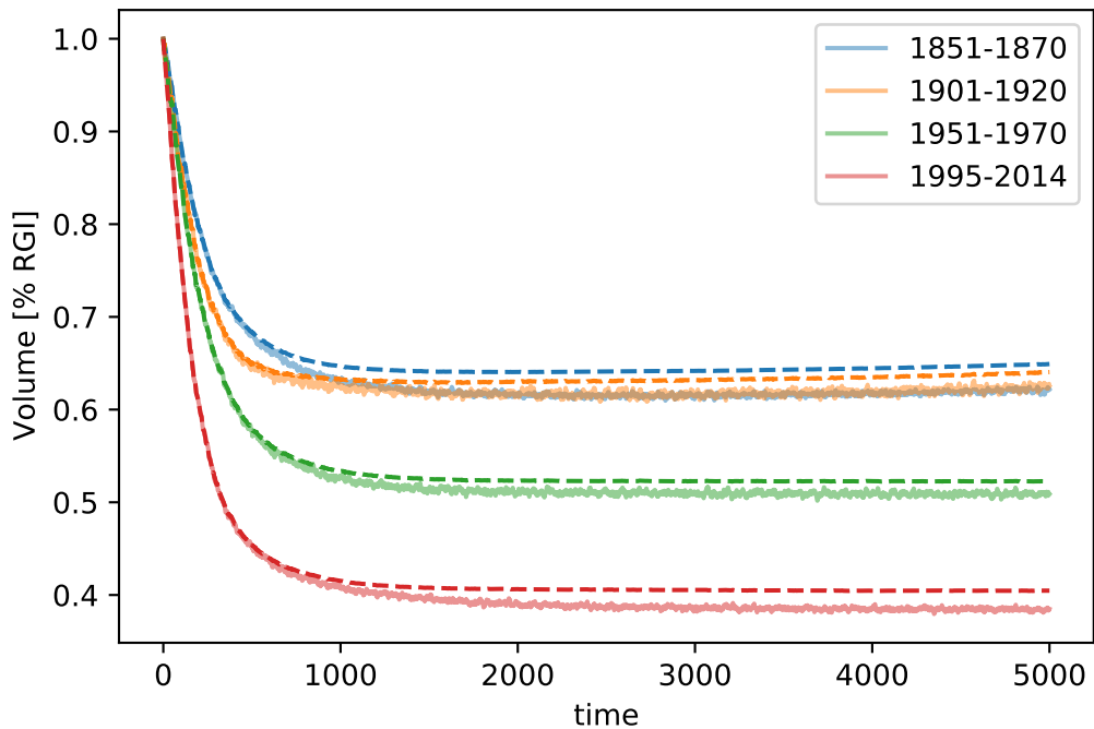
RGI05 (dash=stop). Stop crit 2 (SMB based, 100 yr period)
