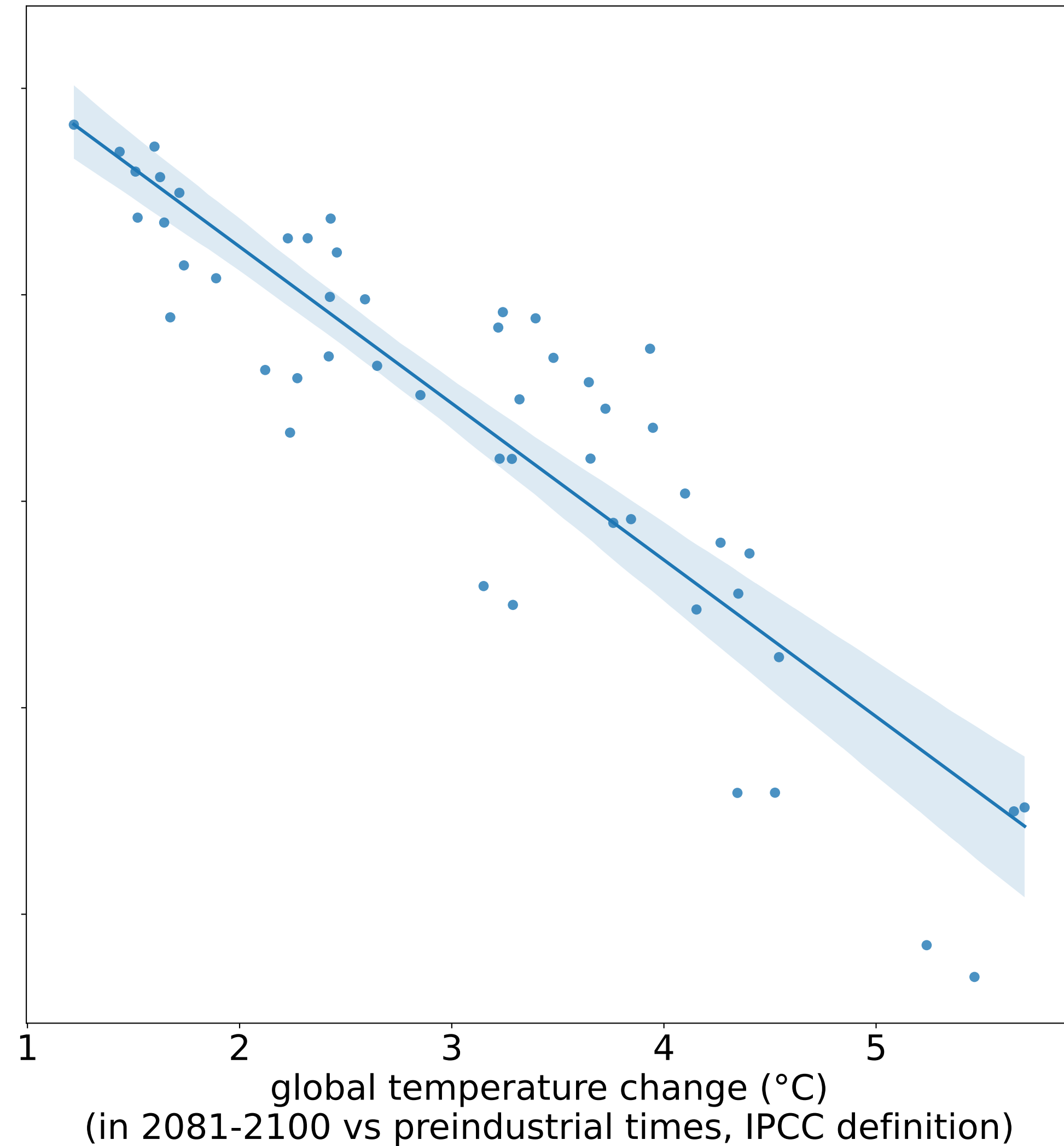
2081-2100: n=51 GCMs & SSPs
