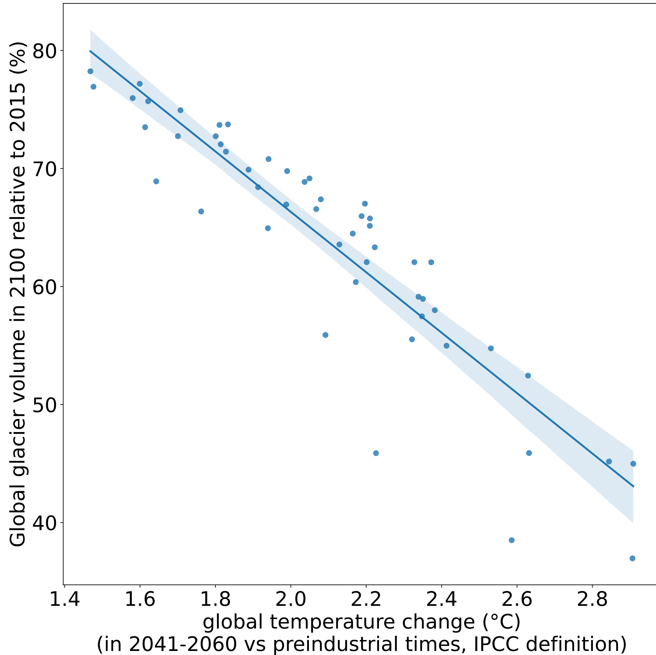
2041-2060: n=51 GCMs & SSPs
